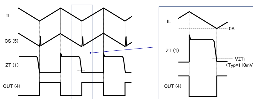
Figure 11. Zero-cross Detection by ZT Pin
