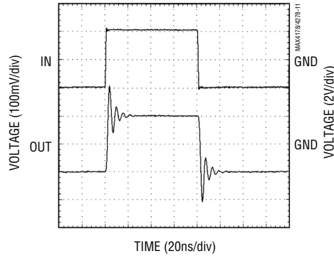
MAX4178 LARGE-SIGNAL PULSE RESPONSE ( C_L = 100pF )
