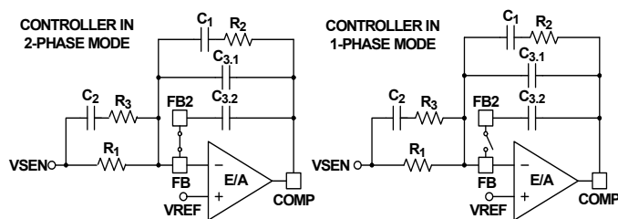
FIGURE 20. FB2 FUNCTION
