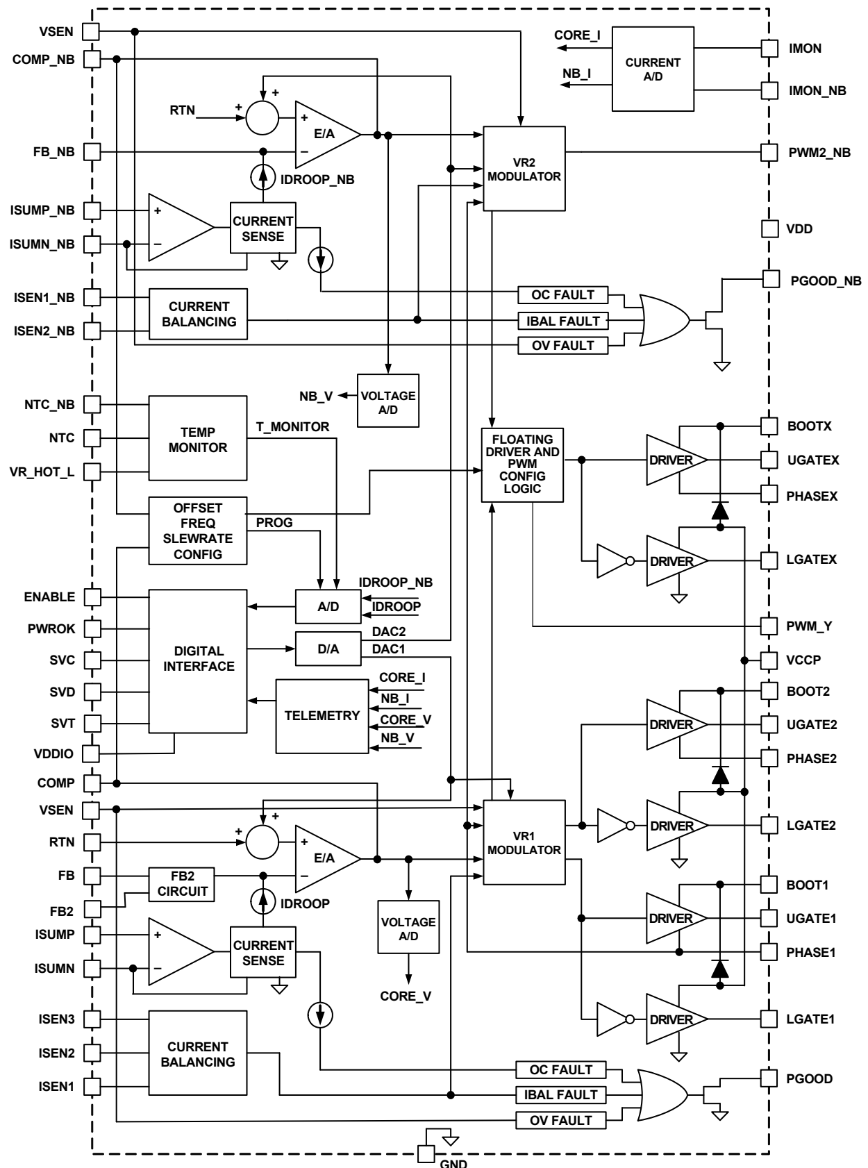
FIGURE 7. BLOCK DIAGRAM
