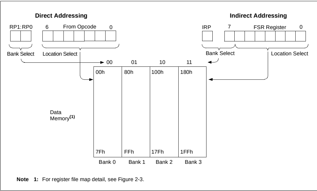
FIGURE 2-5: DIRECT/INDIRECT ADDRESSING
