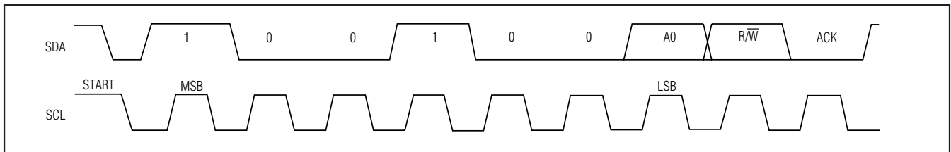
Figure 15. Slave Address
