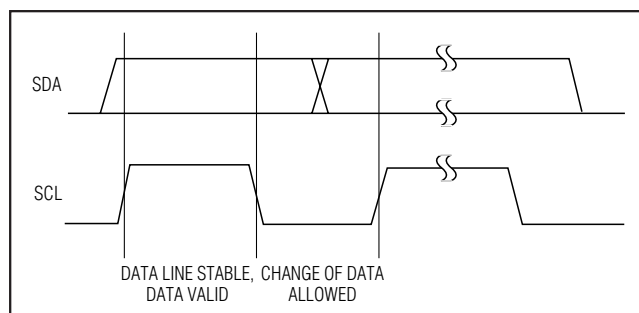
Figure 16. Bit Transfer
