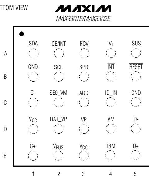
UCSP (2.5mm x 2.5mm)
