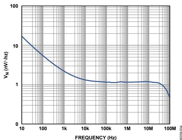
Figure 34. Voltage Noise Spectral Density
