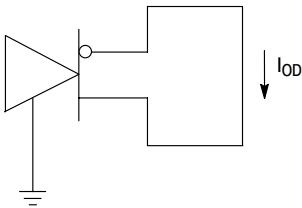
Figure 7. AUI Differential Output Short Circuit Current
