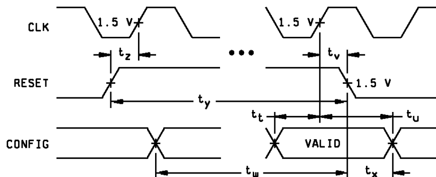
RESET AND CONFIGURATION TIMINGS
