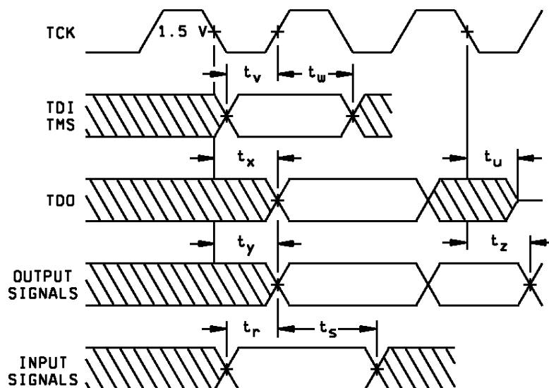
TEST TIMINGS
