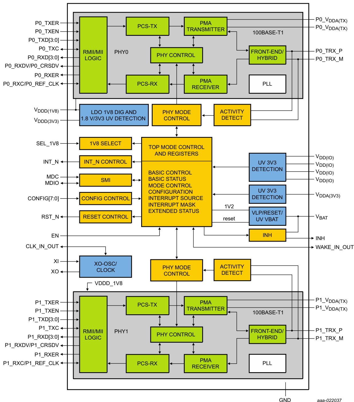
Fig 1. Block diagram (PHY1 is disabled in TJA1102S)
