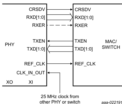
c. Using externally generated 25 MHz reference clock
