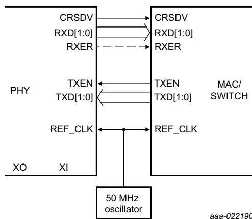
b. Using external reference clock
