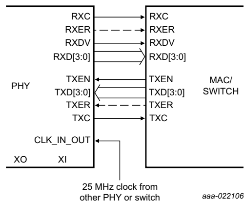
b. Using external reference clock
