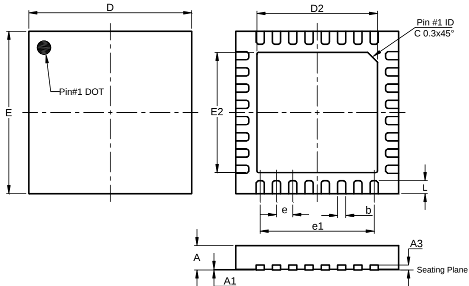
W-QFN5050-32 (Standard)
