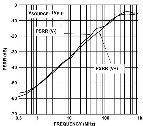
FIGURE 9. PSRR
