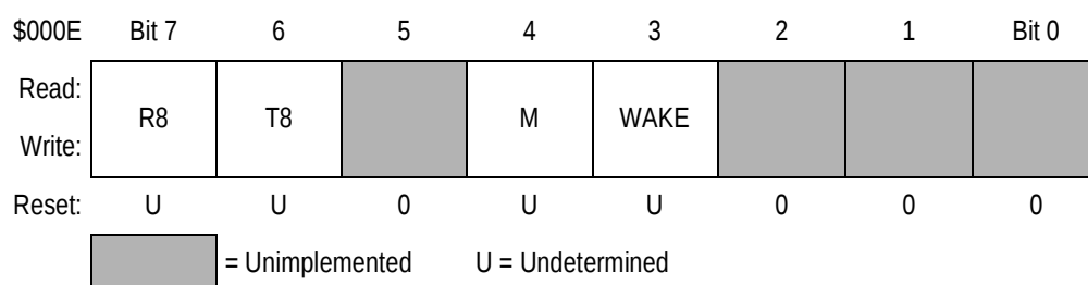
Figure 9-9. SCI Control Register 1 (SCCR1)
