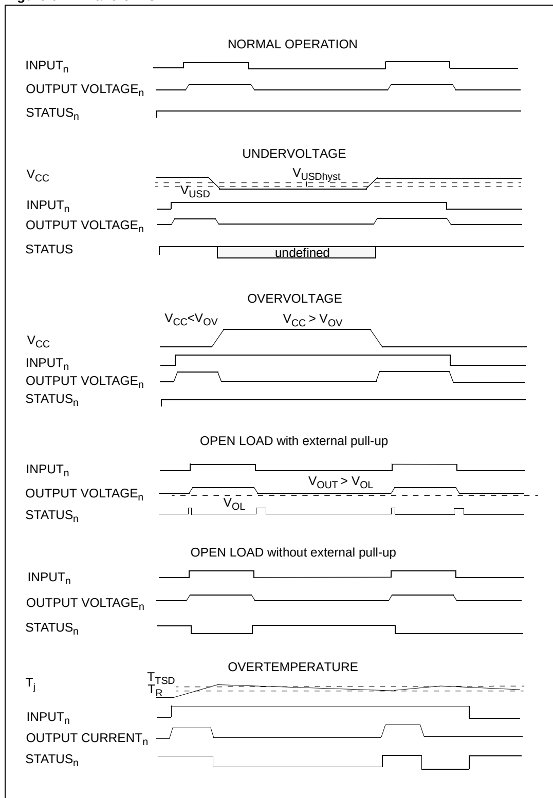
Figure 6. Waveforms
