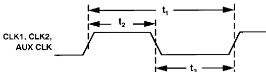
Figure 1. Clock Timing
