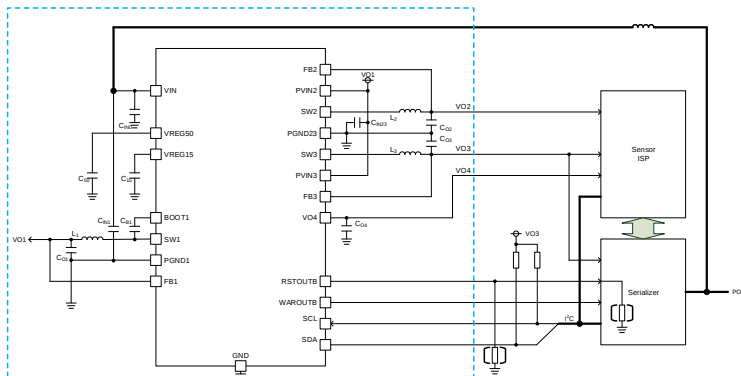
BD868A0 base
