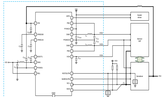
BD868B0 base
