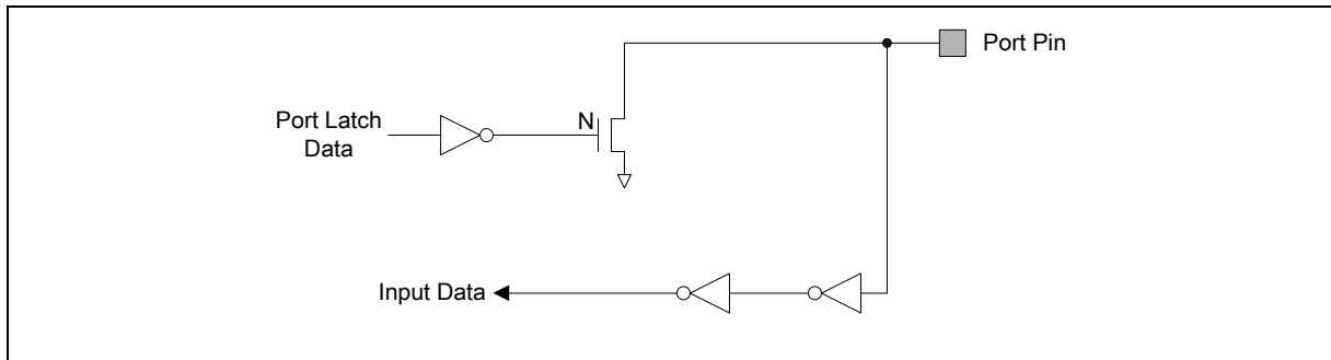
Figure 5-9 Open-Drain Output
