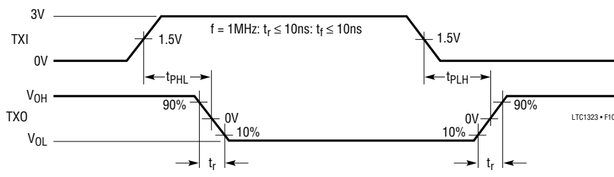
Figure 10. Single-Ended Driver
