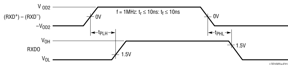
Figure 11. Differential Receiver
