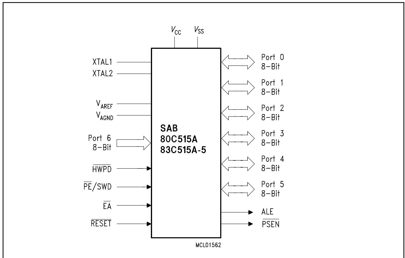
Logic Symbol
