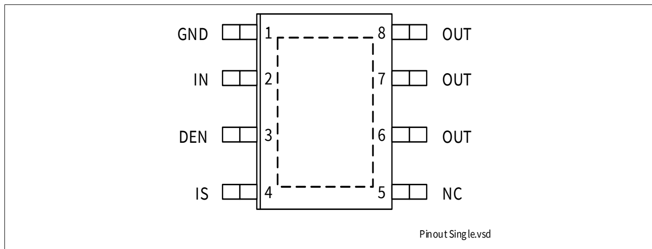
Figure 2 Pin Configuration
