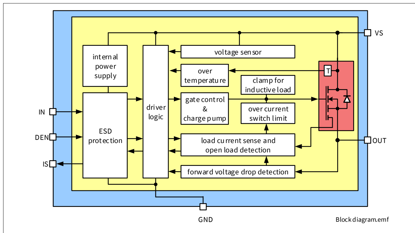
Figure 1 Block Diagram for the BTS5200-1ENA
