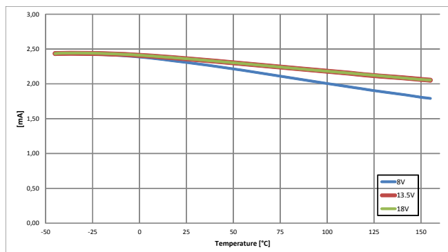
Current Consumption for Whole Device with Load Channel Active I_{GND\_1} = f(T_J; V_S)
