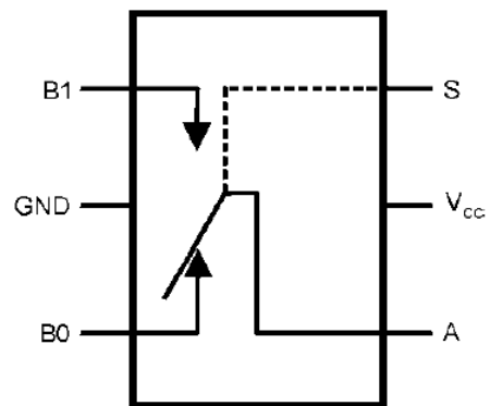
Figure 2. Analog Symbol
