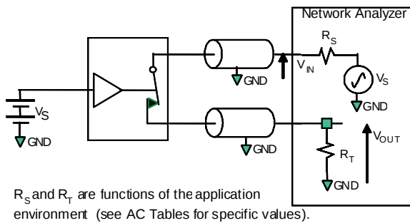
Figure 10. Bandwidth
