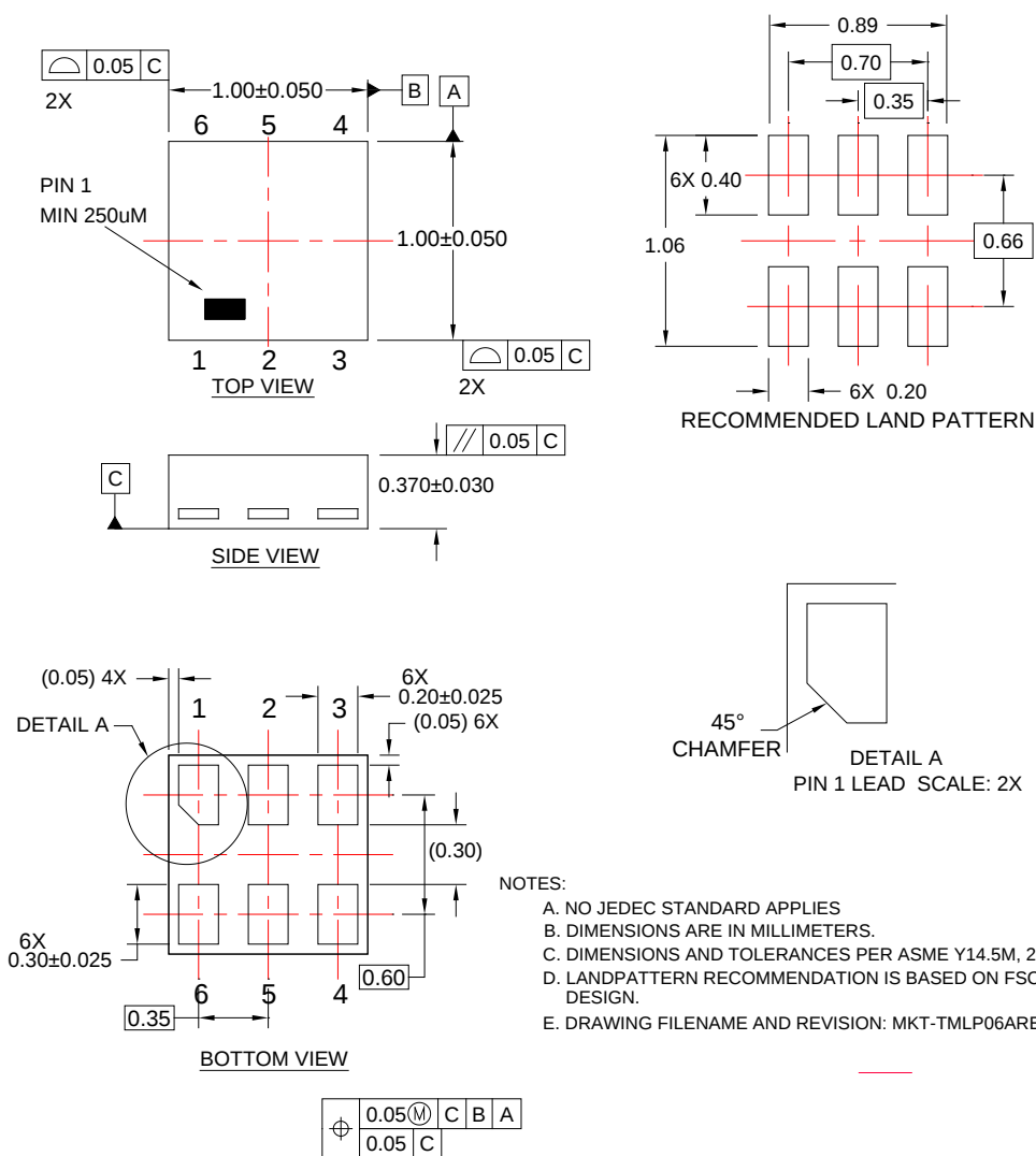
6-Lead, Dual, Ultra-ultrathin Molded Leadless Package (TMLP), 1.0 x 1.0 mm
