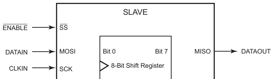
Figure 41. SPI Slave Device
