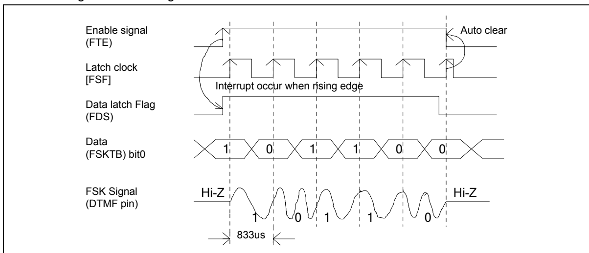
Figure 6-12 FSK Modulator
