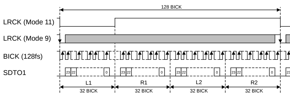
Figure 15. Mode 9/11 Timing (TDM128 mode, I 2 S Compatible)
