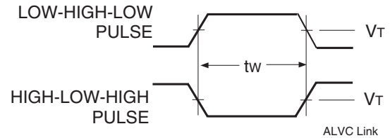
Pulse Width
