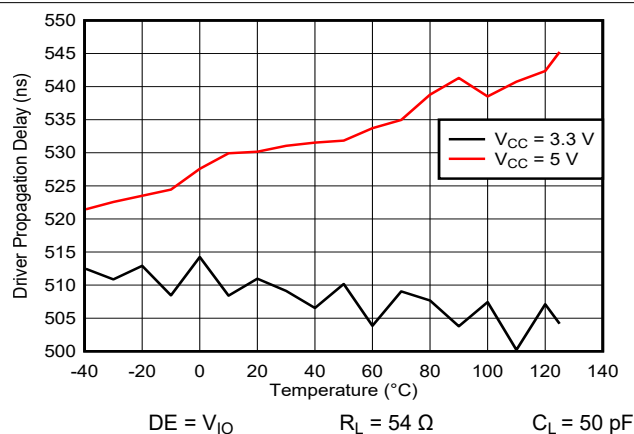
Figure 6-6. THVD2410V 250kbps Driver propagation delay vs Temperature
