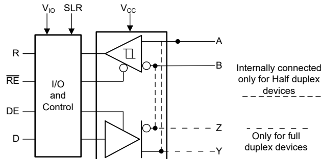
Figure 8-1. THVD2410 and THVD2450 Block Diagram
