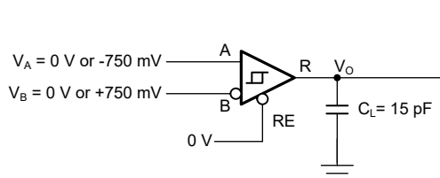
Figure 7-9. Measurement of Fail-Safe Delay
