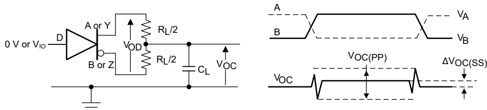
Figure 7-2. Measurement of Driver Differential and Common-Mode Output With RS-485 Load
