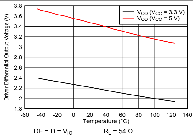
Figure 6-4. Driver differential output voltage vs Temperature
