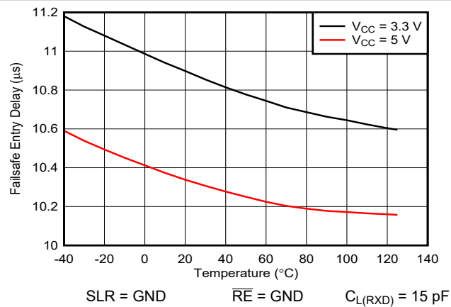
Figure 6-15. Failsafe entry delay vs Temperature
