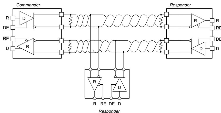
Figure 9-2. Typical RS-485 Network with Full-Duplex transceivers
