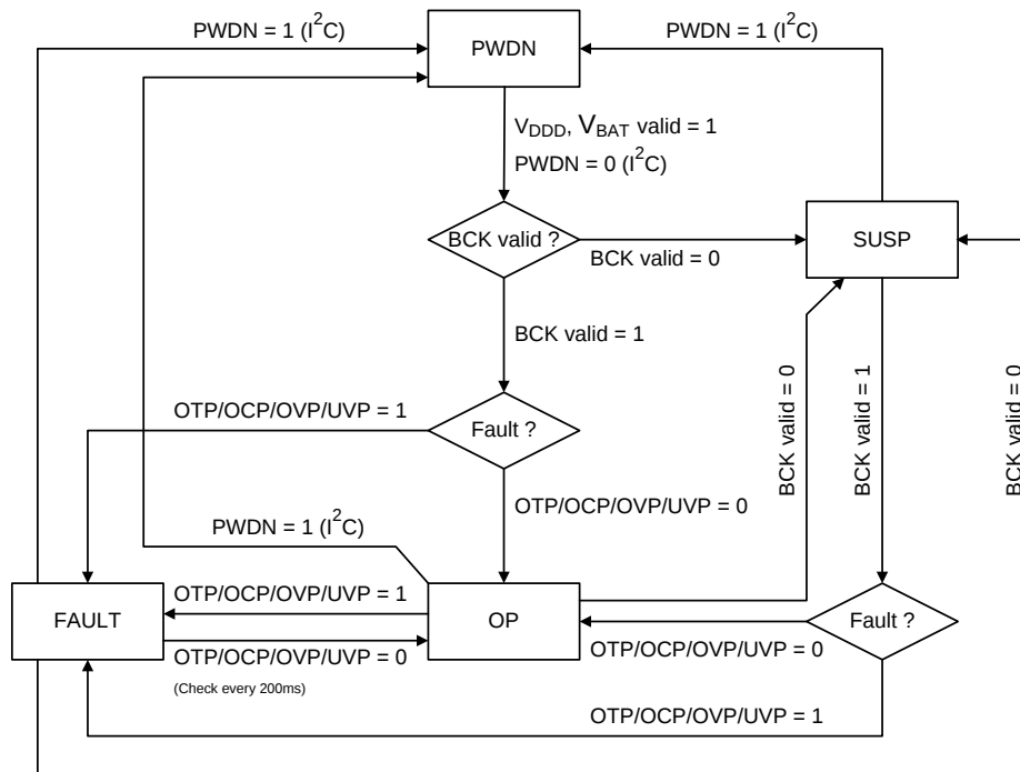
Figure 6. Mode Transition
