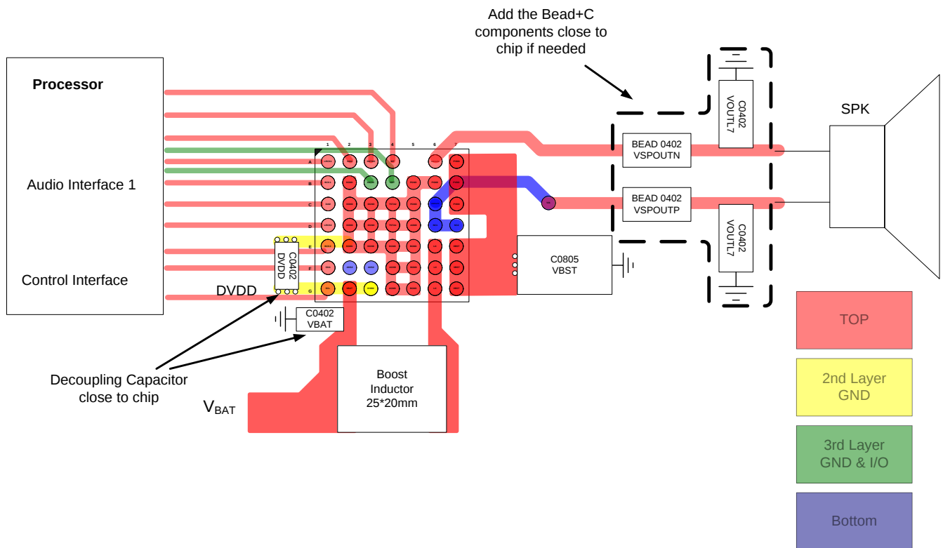
Figure 24. PCB Layout Guide
