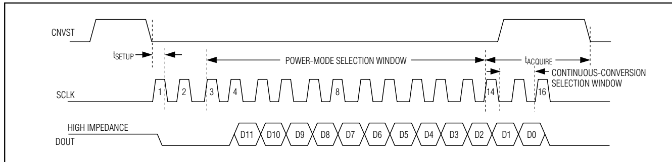
Figure 5. Interface-Timing Sequence
