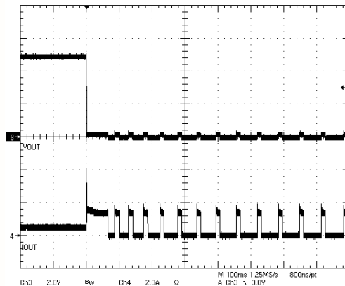
Figure 6. Over-temperature Protection
