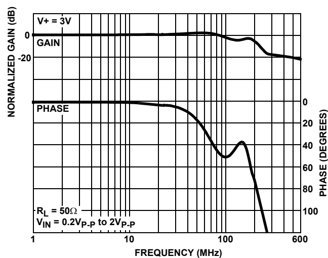
FIGURE 15. FREQUENCY RESPONSE
