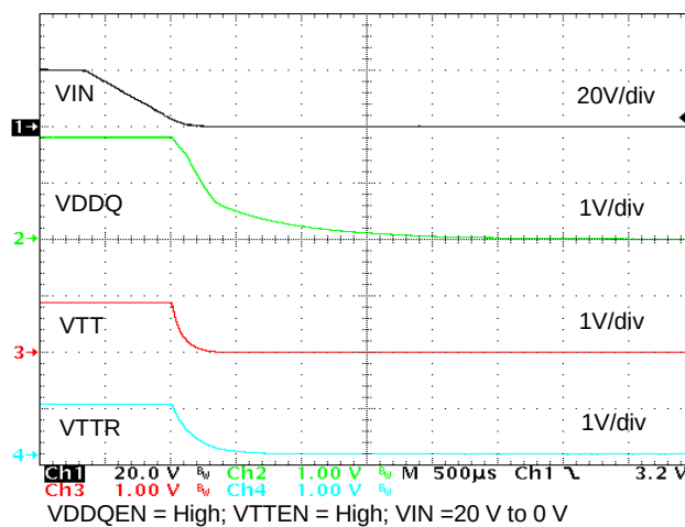
Figure 18. Power-Down Waveforms
