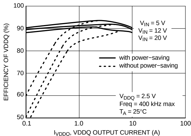
Figure 15. VDDQ Efficiency (DDR) vs. VDDQ Output Current
