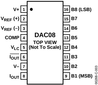
Figure 3. 16-Lead SOIC (S Suffix)
