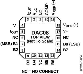
Figure 4. DAC08RC/883 20-Lead LCC (RC Suffix)
