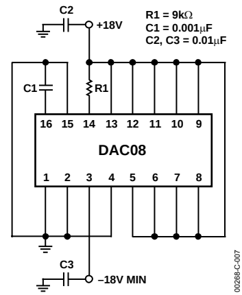
Figure 6. Burn-In Circuit
