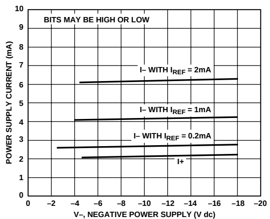
Figure 21. Power Supply Current vs. V-
