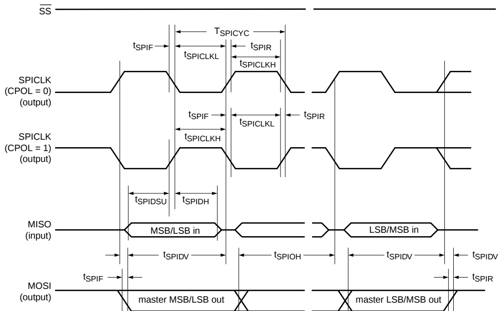
Fig 25. SPI master timing (CPHA = 1)
