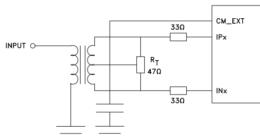
Figure 6: Transformer coupled input
