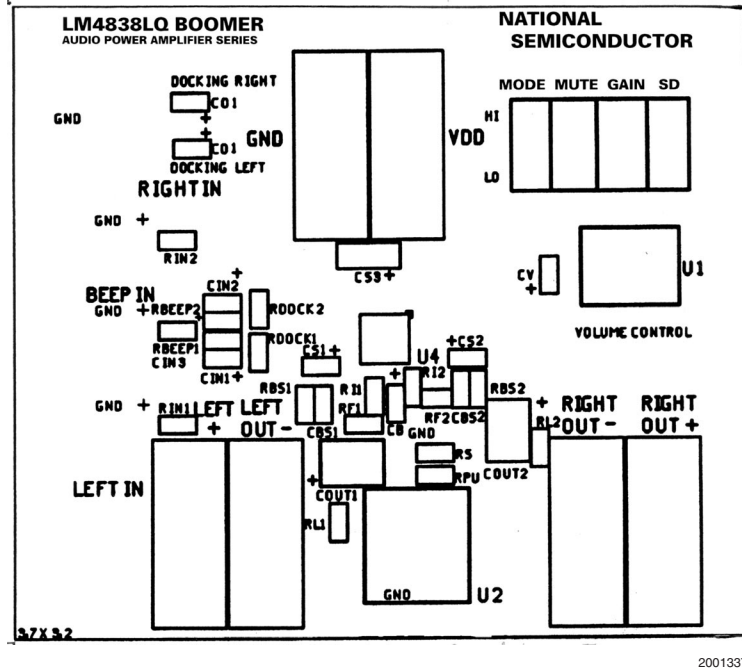
FIGURE 5. Recommended LQ PC Board Layout: Component-Side Silkscreen
