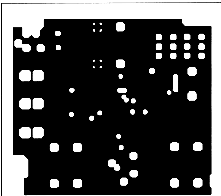
FIGURE 8. Recommended LQ PC Board Layout: Lower Inner-Layer Layout
