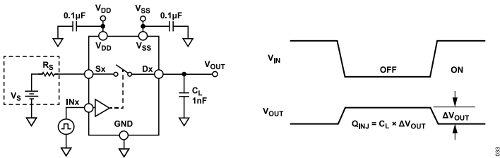
Figure 33. Charge Injection
