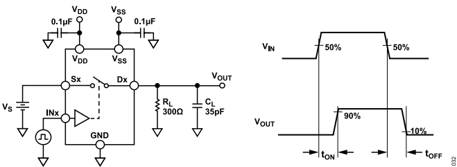
Figure 32. Switching Times
