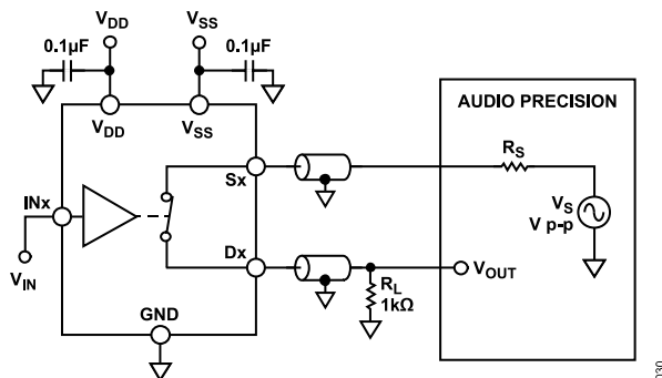
Figure 30. THD + Noise
