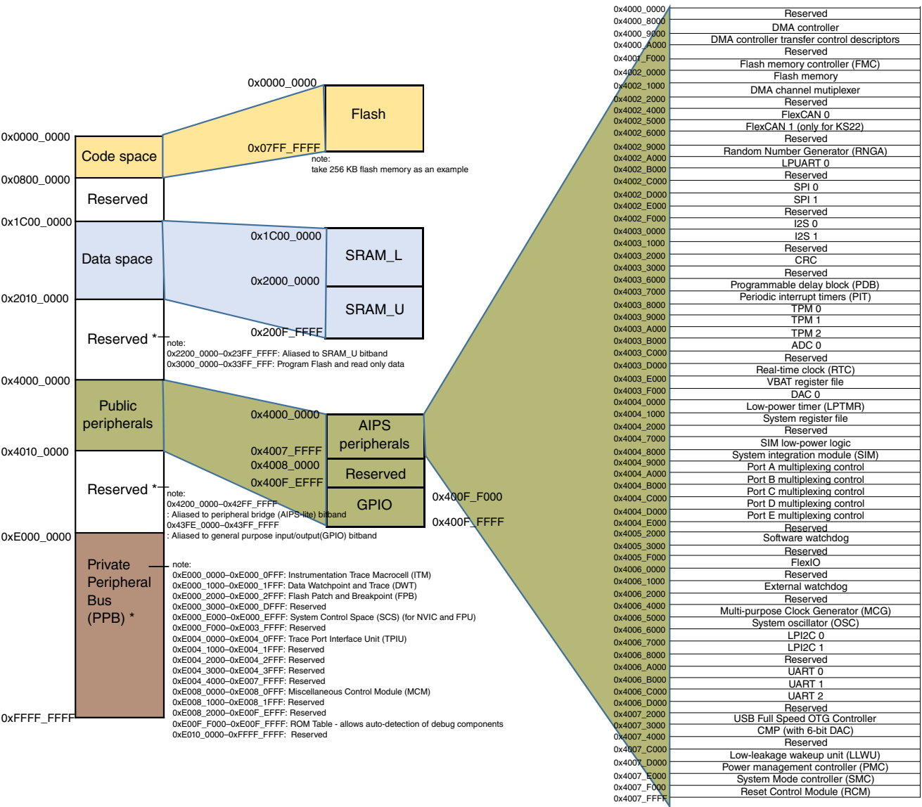
Figure 5. Memory map
