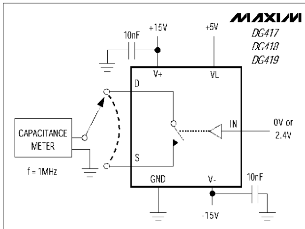
Figure 8. Drain-Source Off-Capacitance
