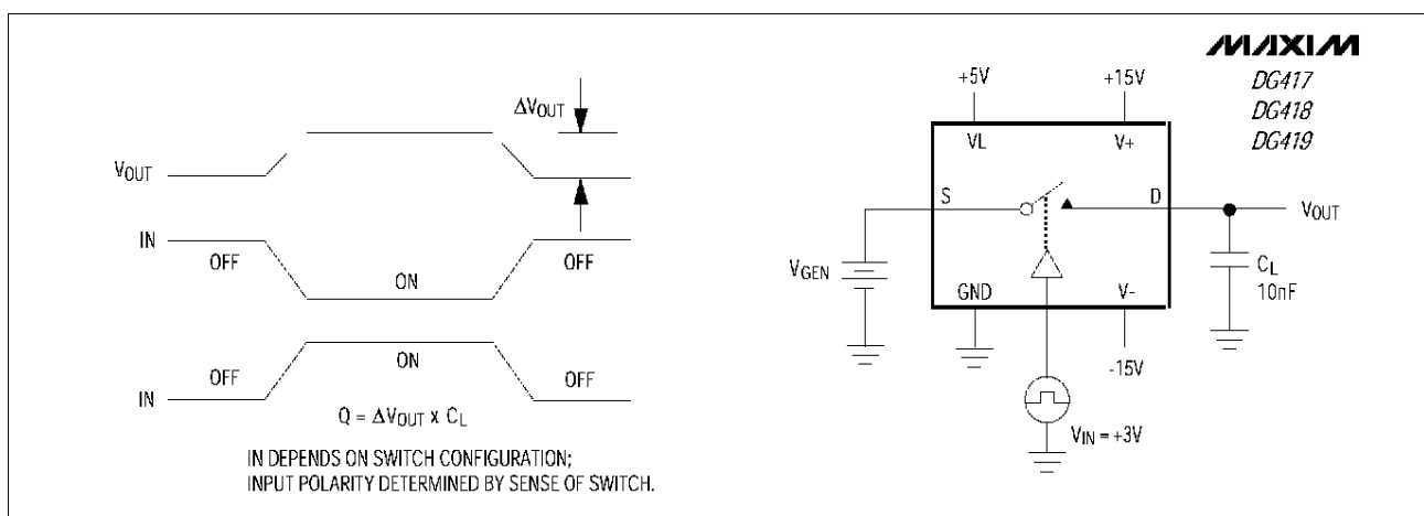
Figure 5. Charge Injection
