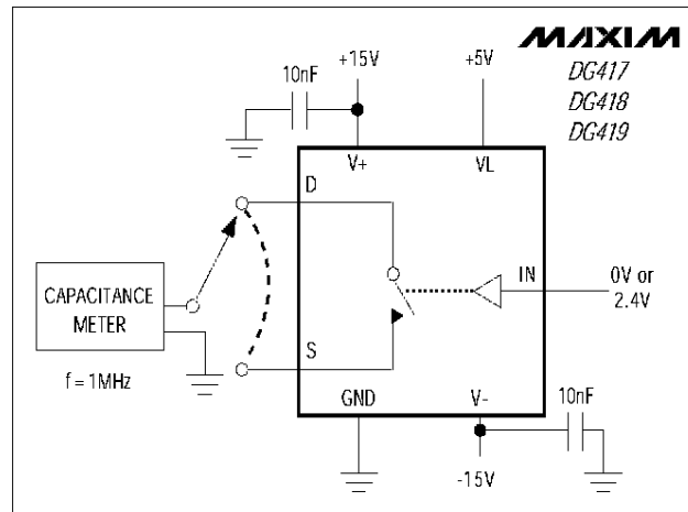
Figure 9. Drain-Source On-Capacitance
