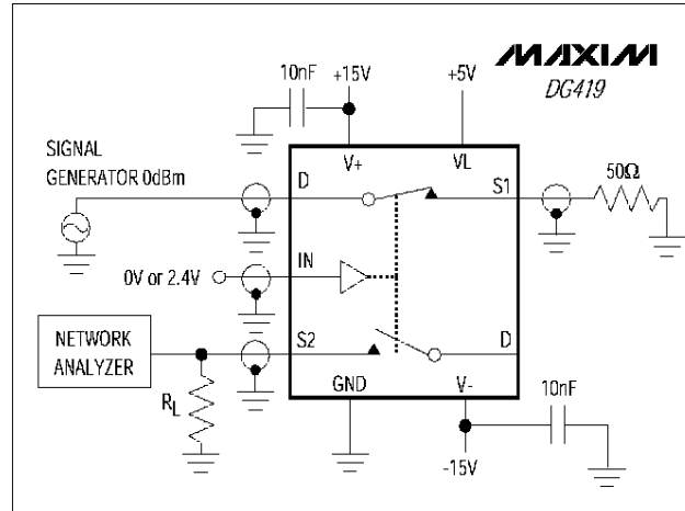
Figure 7. DG419 Crosstalk
