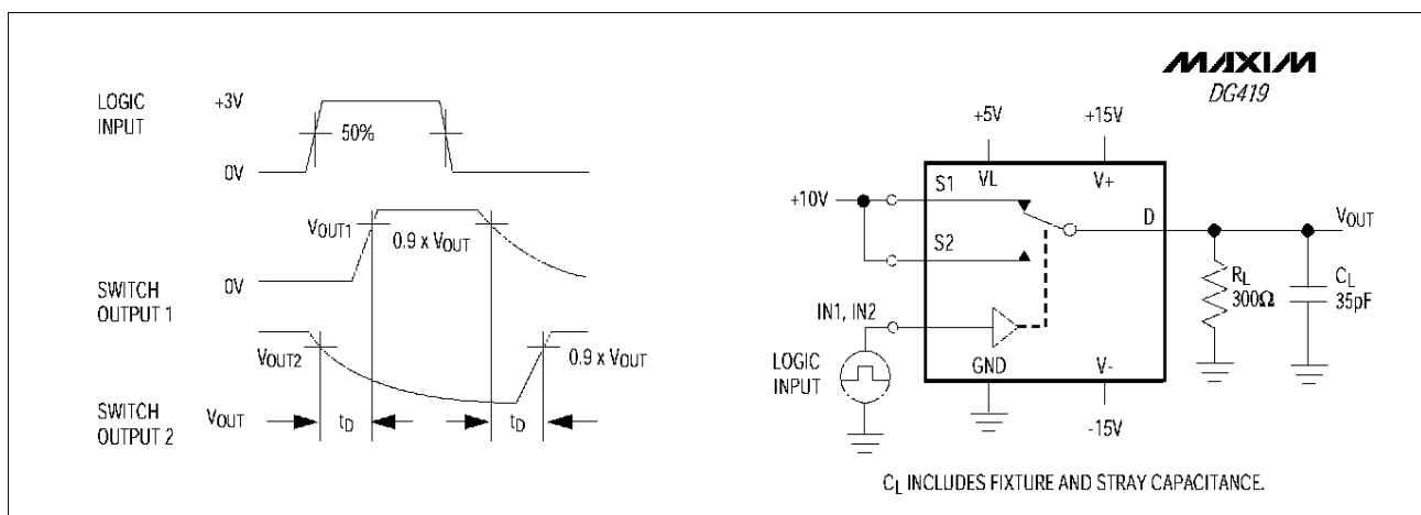
Figure 4. DG419 Break-Before-Make Interval
