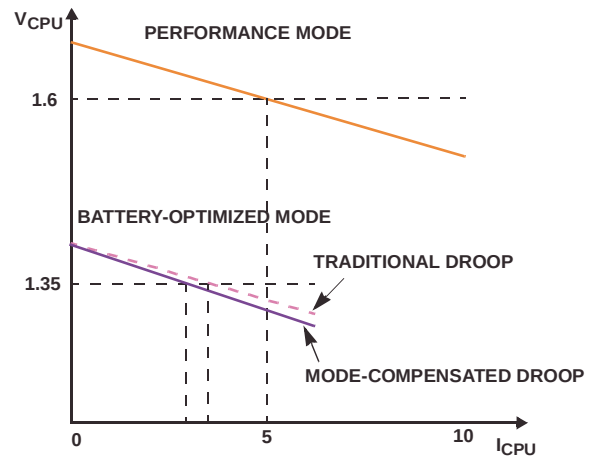
FIGURE 2. MODE-COMPENSATED DROOP
