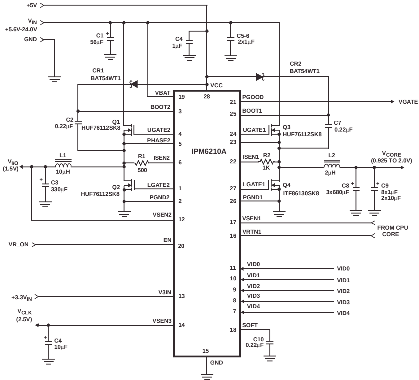
FIGURE 12. APPLICATION CIRCUIT
