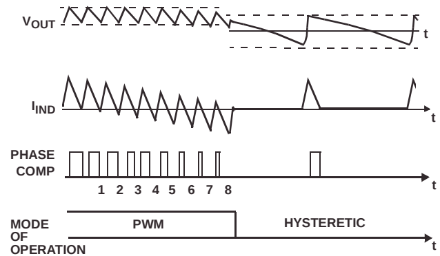
FIGURE 7. PWM TO HYSTERETIC TRANSITION
