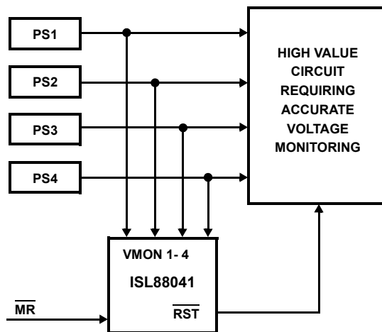
FIGURE 9. TYPICAL ISL88041 APPLICATION DIAGRAM
