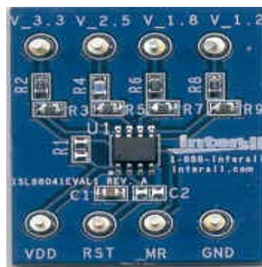
FIGURE 11. ISL88041EVAL1 PHOTO
