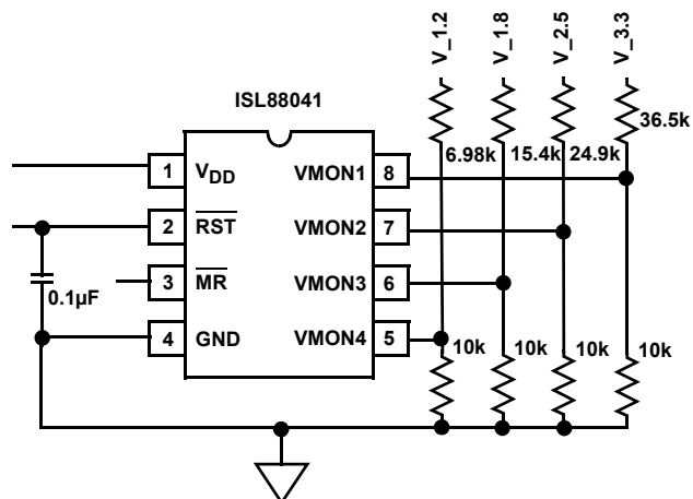
FIGURE 10. ISL88041EVAL1 SCHEMATIC
