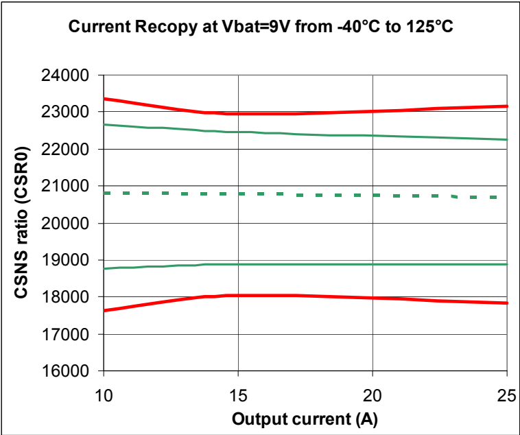
Figure 14. CSR0 Ratio Deviation in Function Manufacturing and Temperature
