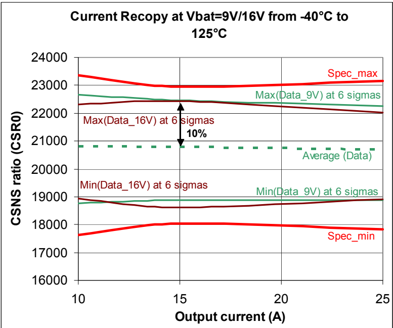
Figure 13. CSR0 Ratio Deviation in Function All Contributors
