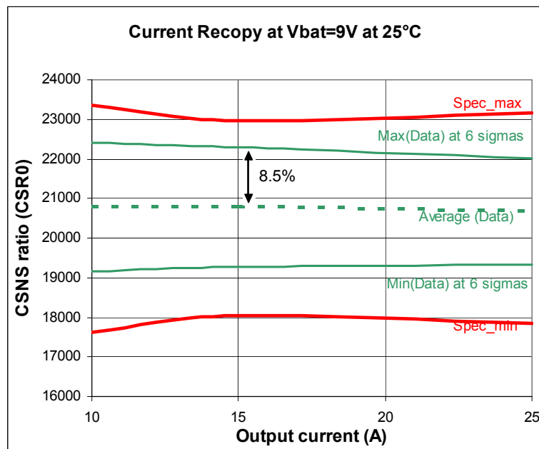
Figure 15. CSR0 Ratio Deviation in Function Manufacturing
