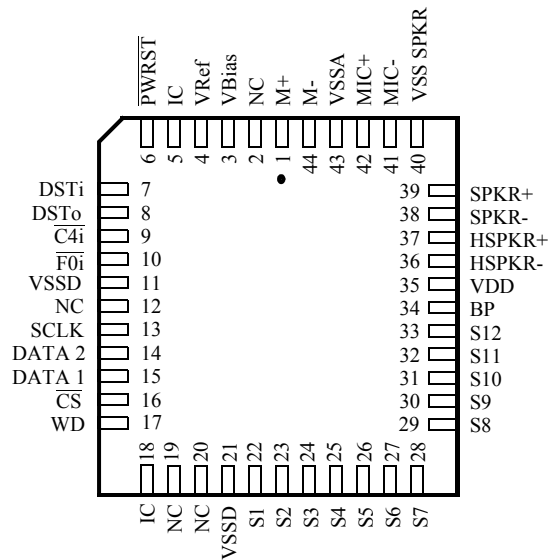
44 PIN PLCC
