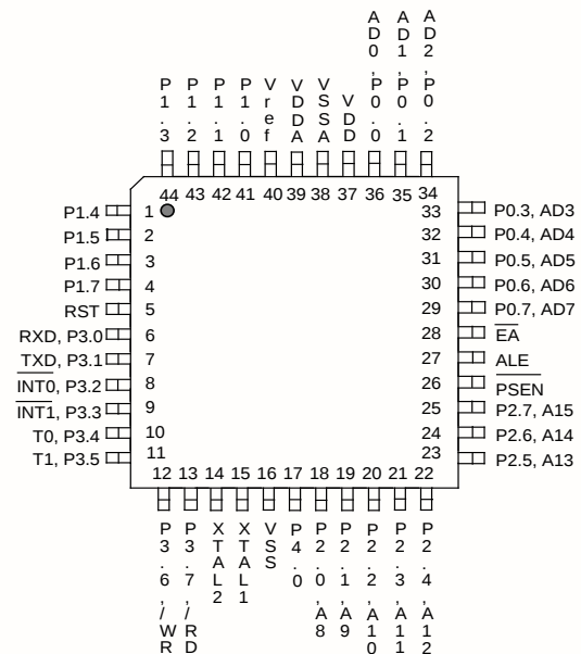
44-Pin QFP
