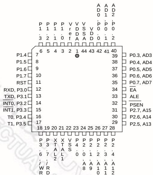
44-Pin PLCC
