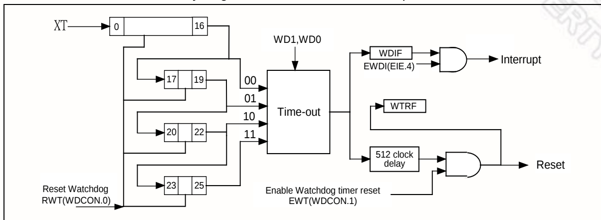
Figure 11-1 Watchdog Timer
