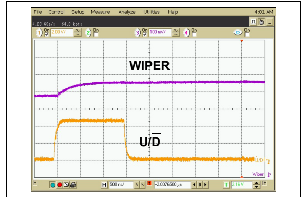
FIGURE 2-29: 5\text{ k}\Omega – Low-Voltage Increment Wiper Settling Time ( V_{DD} = 5.5\text{V} ).
