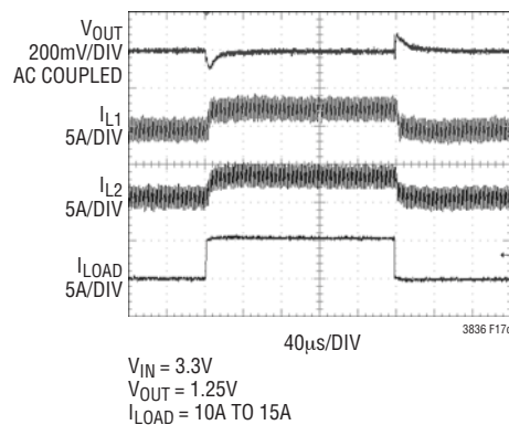
Figure 17c. Load Step
