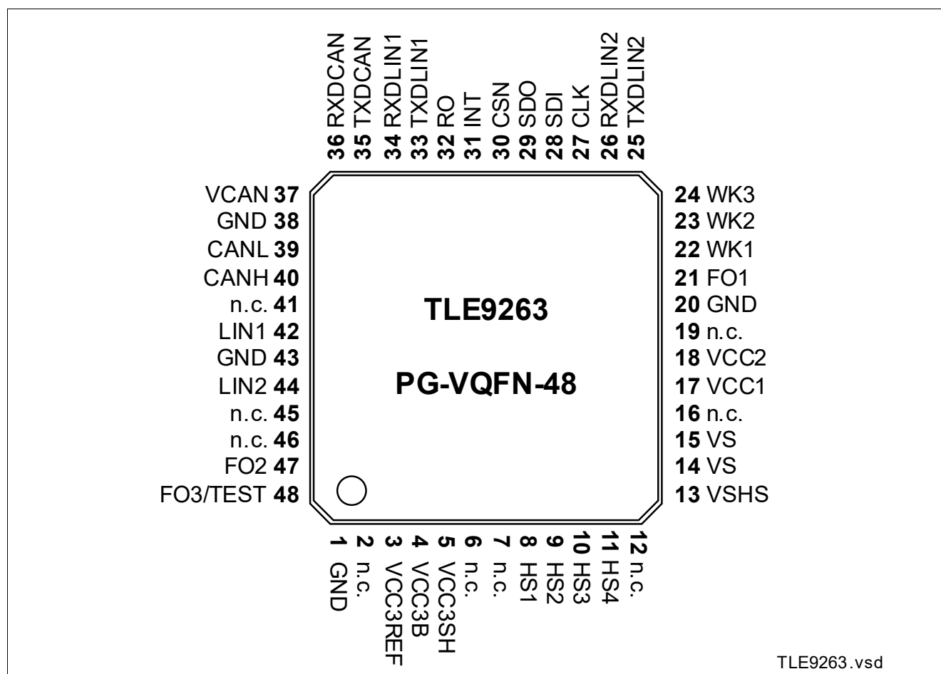
Figure 2 Pin Configuration
