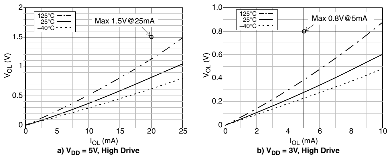
Figure A-1. Typical V_{\text{OL}} vs I_{\text{OL}} , High Drive Strength
