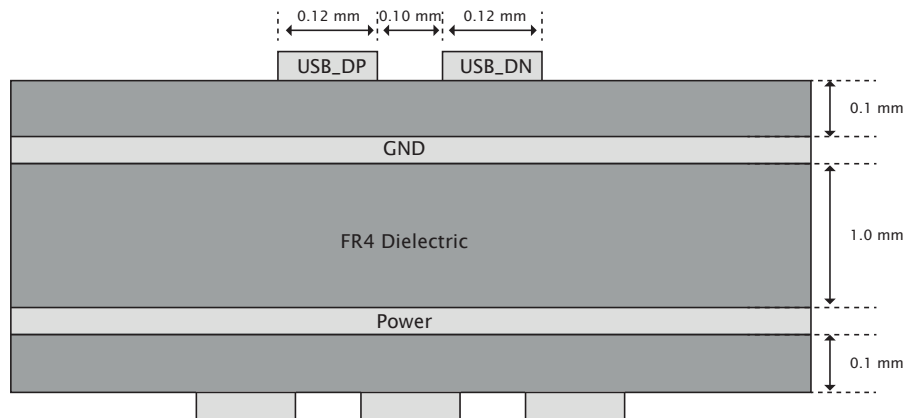
Figure 17: Example USB board stack
