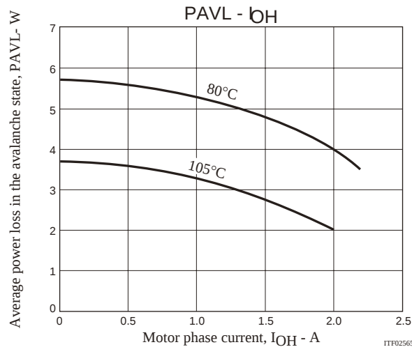
Figure 3 Allowable Loss Range, PAVL-I_{OH} During STK672-530 Avalanche Operations
