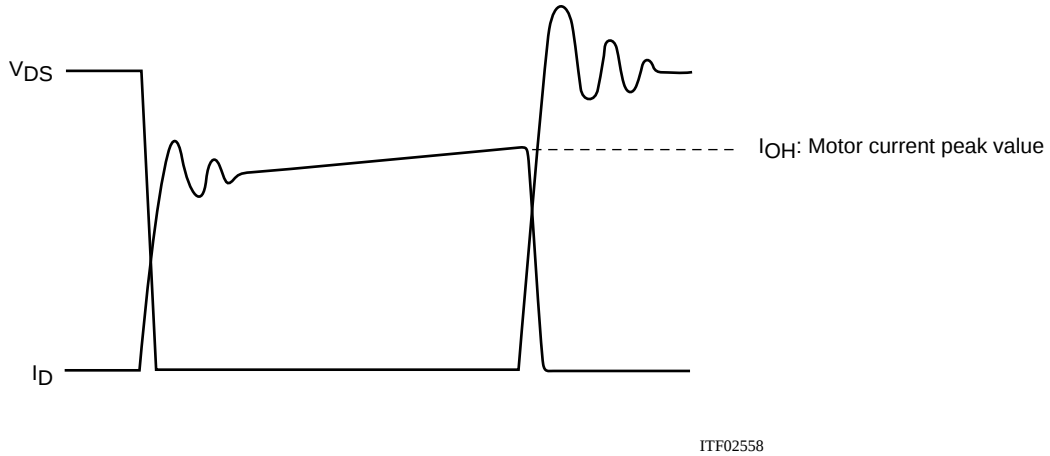
Figure 2 Output Current, I_D , and Voltage, V_{DS} , Waveforms 2 of the STK672-5** Series when Driving a 2-Phase Stepping Motor with Constant Current Chopping
