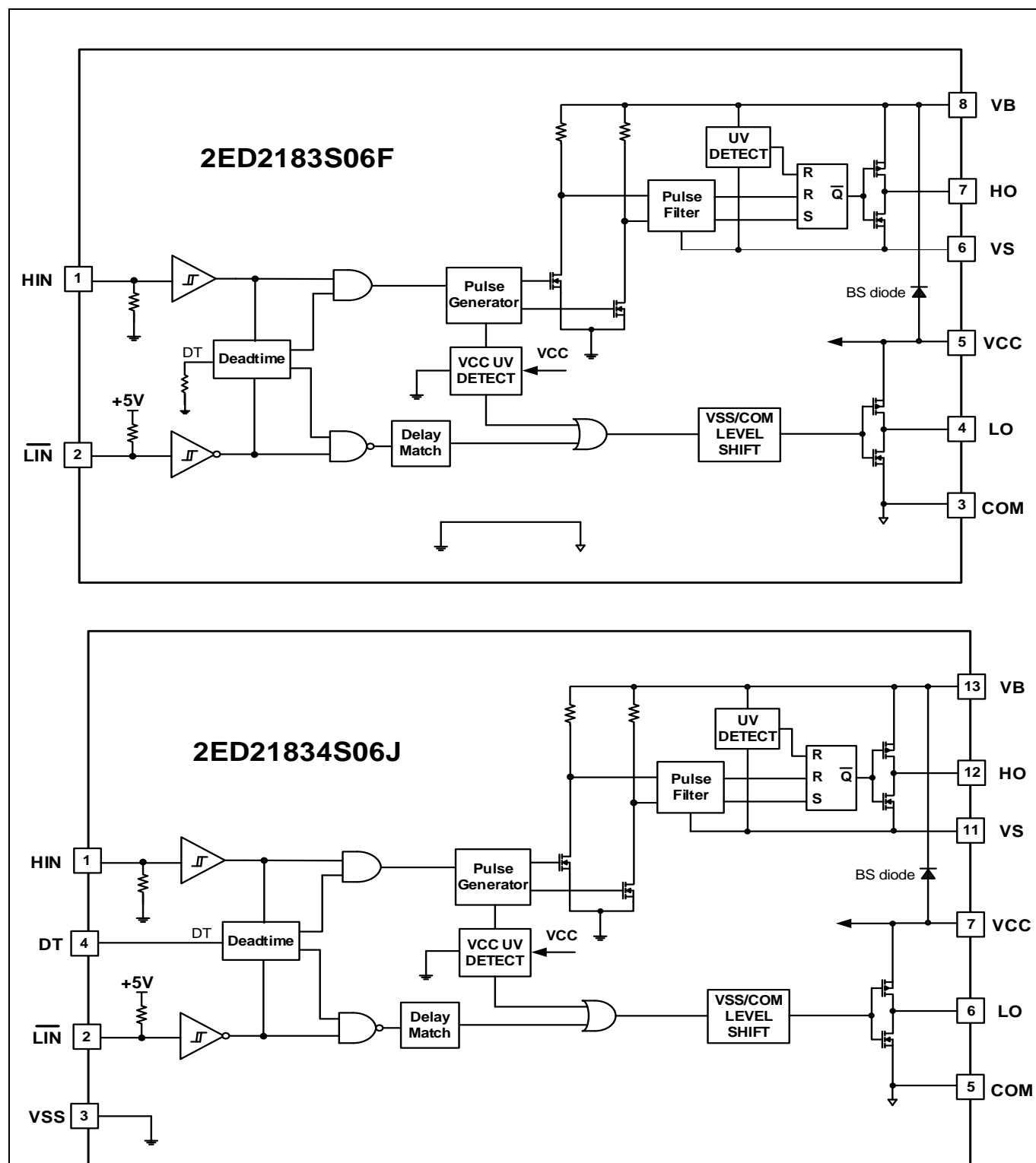
Figure 2 Block diagrams
