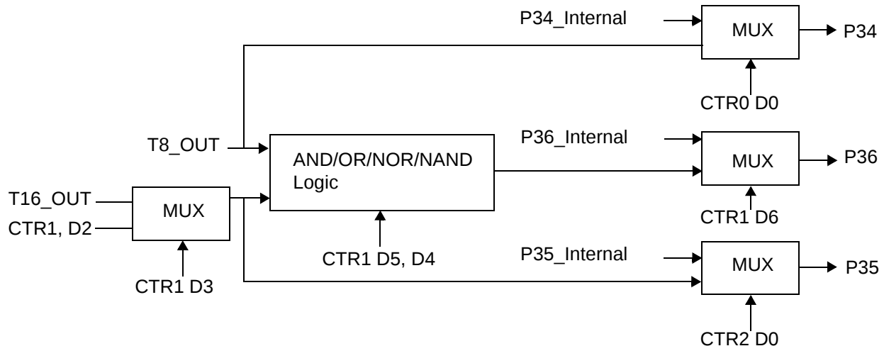
Figure 26. Output Circuit
